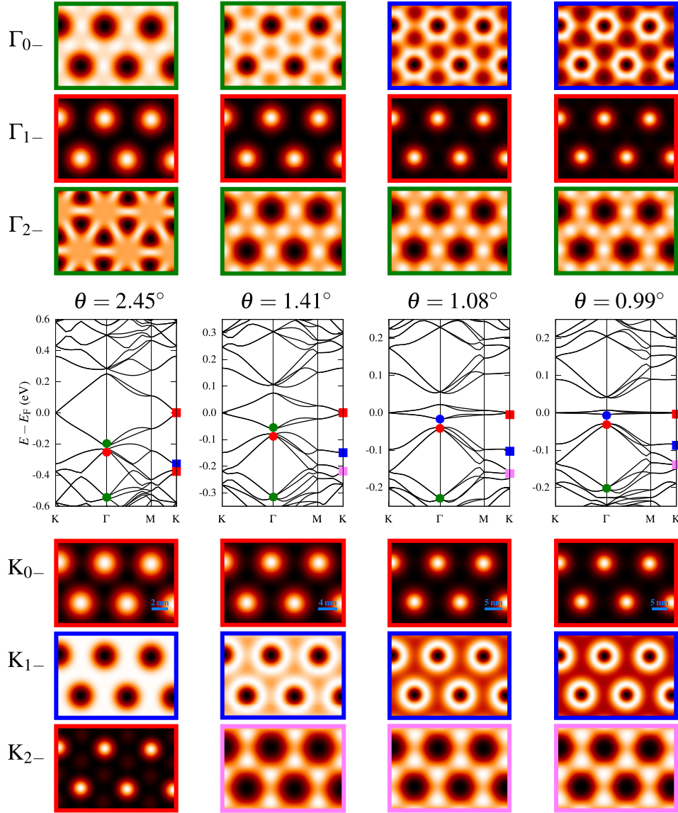
FIG. 8. Electronic band structures and wave functions as a function of twist angle \theta . The points \Gamma_{n-} ( K_{n-} ), where n = 0, 1, 2 , are shown are highlighted on the band structures by the circles (squares), and the corresponding wave functions are shown above (below) the band structures. The color of the markers on the band structures and the borders of the wave functions indicates the character of the wave functions as described in the text.
