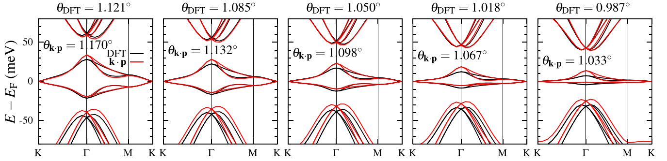
FIG. 5. Electronic band structure of tBLG for commensurate twist angles near the magic angle. The black lines show the bands from DFT calculations with SIESTA and the red lines show the bands obtained using the \mathbf{k} \cdot \mathbf{p} model. A small shift of the twist angle used in the \mathbf{k} \cdot \mathbf{p} calculation, \theta_{\mathbf{k} \cdot \mathbf{p}} = \theta_{\text{DFT}} + \Delta\theta where \Delta\theta \approx 0.05^\circ , improves the agreement with the DFT bands.
