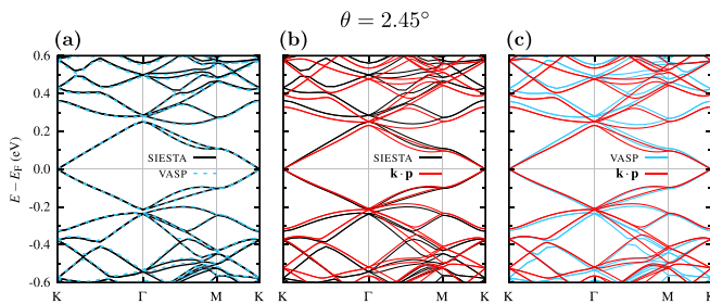
FIG. 4. Comparison of electronic band structure of tBLG for \theta = 2.45^\circ calculated using SIESTA, VASP, and the \mathbf{k} \cdot \mathbf{p} model. The black lines show the bands from DFT calculations with SIESTA, the blue lines show the bands from DFT calculations with VASP, and the red lines show the bands obtained using the \mathbf{k} \cdot \mathbf{p} model.
