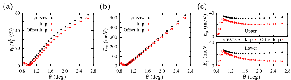
FIG. 6. (a) Fermi velocity as a function of twist angle from SIESTA (black) and the exact \mathbf{k} \cdot \mathbf{p} model (red), as a percentage of the Fermi velocity of graphene, v_F^0 = 1 \times 10^6 m/s. For the \mathbf{k} \cdot \mathbf{p} model, filled circles correspond to initial twist angles \theta_{\mathbf{k} \cdot \mathbf{p}} , while open circles correspond to \mathbf{k} \cdot \mathbf{p} twist angles that have been shifted by \Delta\theta \approx 0.05^\circ towards smaller angles. (b) Band width E_w (meV) at \Gamma as a function of twist angle from SIESTA (black) and the exact \mathbf{k} \cdot \mathbf{p} model (red). (c) Band gaps E_g (meV) between the flat and dispersive bands at \Gamma as a function of twist angle from SIESTA (black) and the exact \mathbf{k} \cdot \mathbf{p} model (red). The upper (lower) panel corresponds to the gap above (below) the Fermi level.
