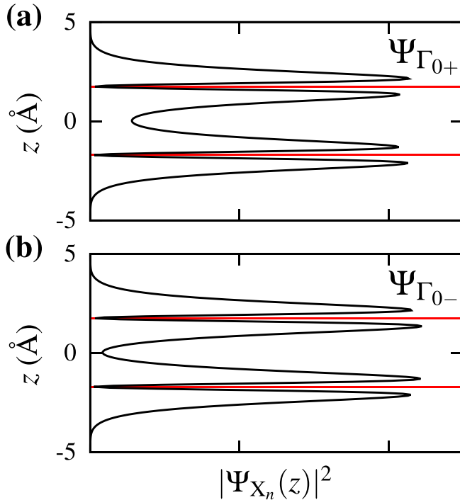
FIG. 7. Probability density of the (a) \Gamma_{0+} and (b) \Gamma_{0-} wave functions of magic-angle tBLG (1.08°) in the out-of-plane direction, averaged over the in-plane directions. The red lines indicate the average vertical positions of the two layers.
