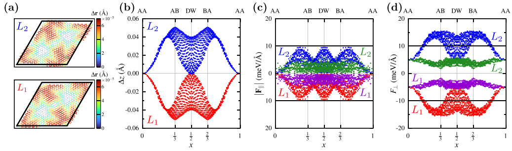
FIG. 1. Comparison of the atomic structure and forces from DFT calculations using SIESTA and VASP, for tBLG with a twist angle of \theta = 2.45^\circ and a monolayer lattice constant of a_0 = 2.46 \text{ \AA} . (a), (b) The difference in positions obtained from SIESTA and VASP. (a) The in-plane direction ( \Delta \mathbf{r} ). The in-plane displacements owing to relaxation are on the order of 10^{-2} \text{ \AA} for both codes, and the difference \Delta \mathbf{r} is less than 1% of the relaxation. (b) The out-of-plane direction ( \Delta z ), projected onto the unit-cell diagonal, where the top layer is shown in blue and the bottom layer in red. (c), (d) The forces obtained from VASP using the relaxed coordinates determined by SIESTA (red/blue) and VASP (green/purple) are shown for: (c) the in-plane direction ( \mathbf{F}_{||} ); (d) the out-of-plane direction ( F_{\perp} ), projected onto the unit cell diagonal. The horizontal black lines show the force tolerance used in the VASP relaxation ( 10 \text{ meV/\AA} ).
