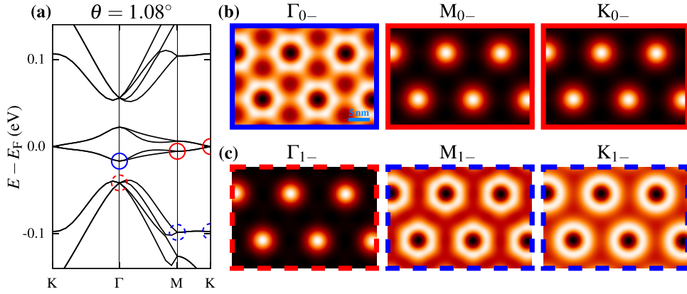
FIG. 9. (a) Band structure of tBLG at the magic angle ( \theta = 1.08^\circ ). (b), (c) Moiré-scale wave functions in (b) the lower flat band, and (c) the dispersive valence band, at the high-symmetry \mathbf{k} -points \Gamma , M , and K . The panel borders match the respective location of the wave functions in the band structure, with solid (dashed) lines representing flat (dispersive) bands, and red and blue indicating wave functions that have AA and AA_z character, respectively.
